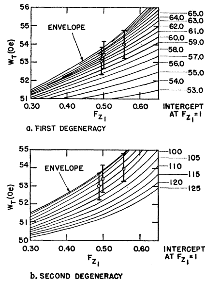
FIG. 3. Expanded combined ESR derivative width extrapolation curves for Z_1 and F centers.
