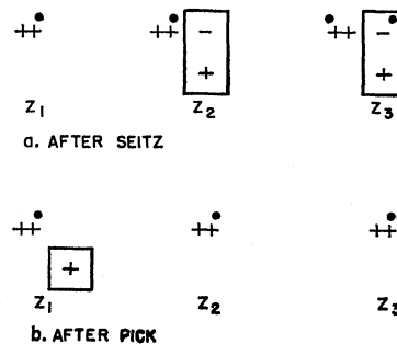
FIG. 1. Proposed Z -center models. The square boxes represent vacancies, \bullet\bullet represents a substitutive divalent ion, and \bullet represents a trapped electron.
